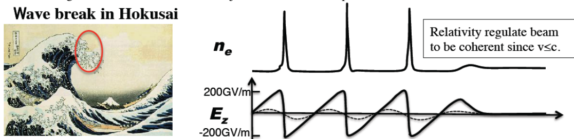
Figure 1: Hokusai's wave breaks but Tajima's wakefield will not break due to relativistic effect.
