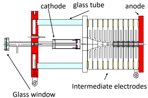
Figure 1. Schematic of the cascade arc device.
