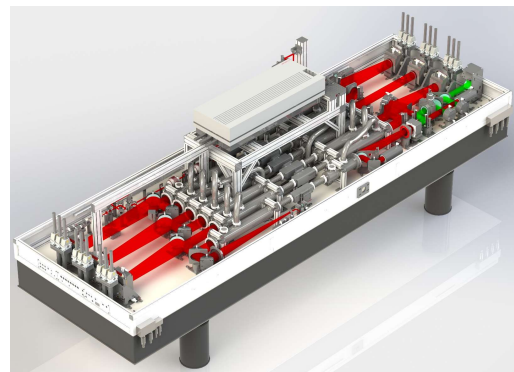
Figure 2: Premiumlite- 50J @10Hz pump laser
