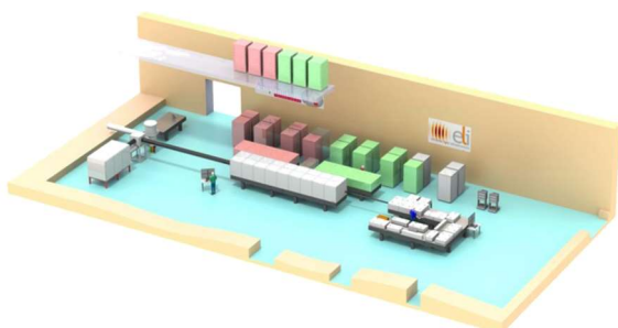
Figure 1: HF laser system, 3D layout
