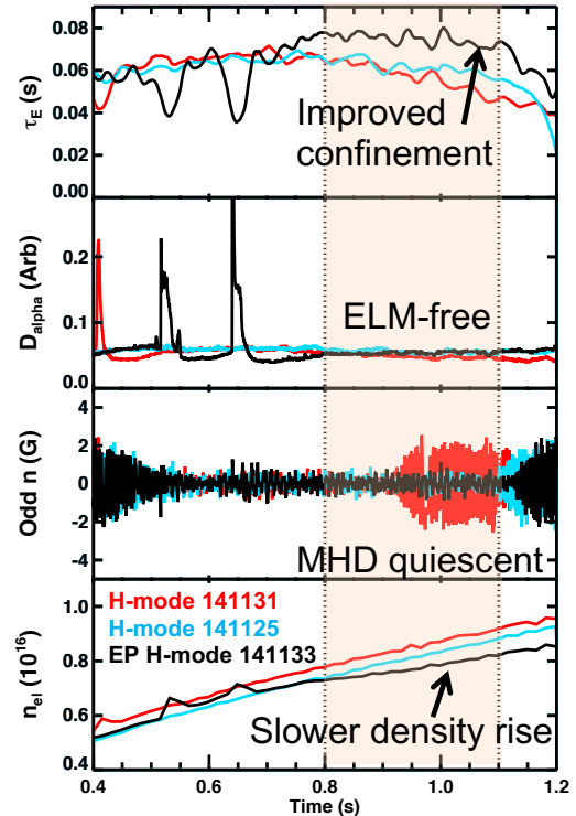
Figure 1 EP H-mode discharge (black) compared to similar ELM-free H-mode discharges (red and blue).
