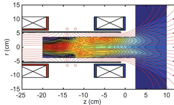
Fig.1: Calculated magnetic field lines and measured ion saturation current of the magnetic nozzle rf plasma thruster providing 30 % efficiency.
